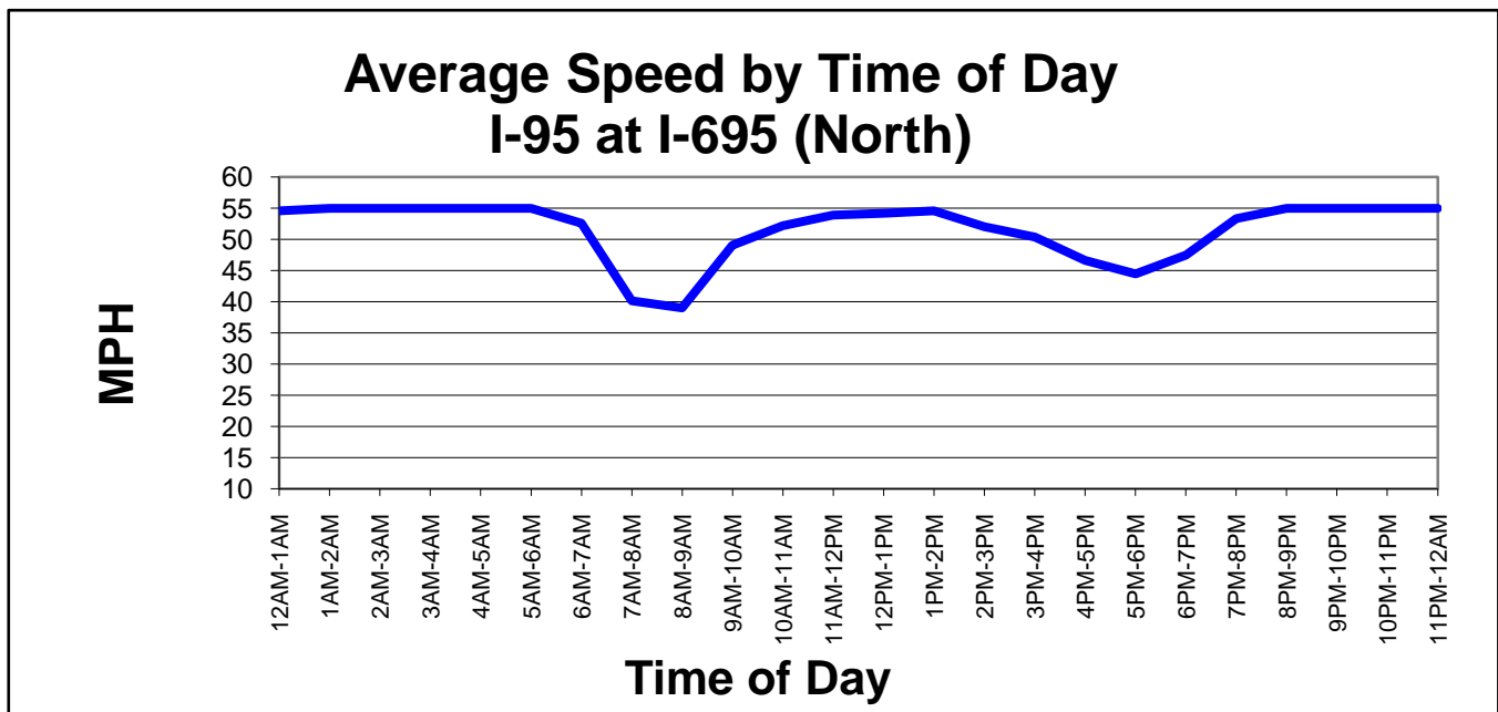
Figure 2: Speed Profile
