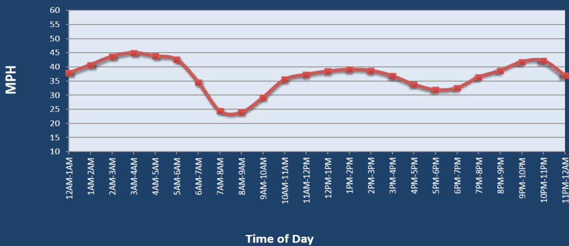
Average Speed by Time of Day I-95 at SR 4
