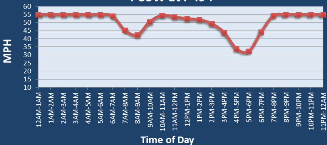
Average Speed by Time of Day I-35W at I-494
