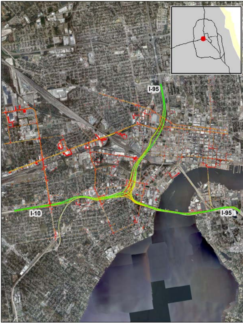
Average Speed by Time of Day I-10 at I-95
