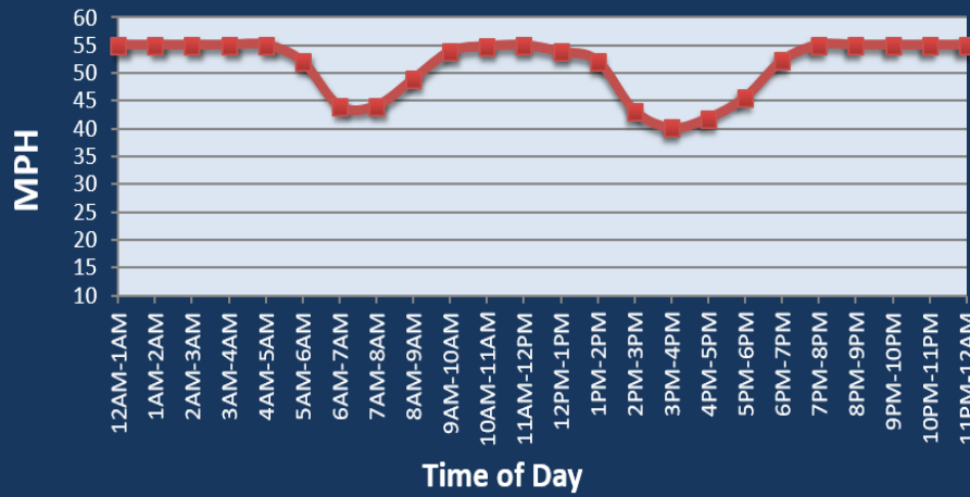
Average Speed by Time of Day SR 18 at SR 167
