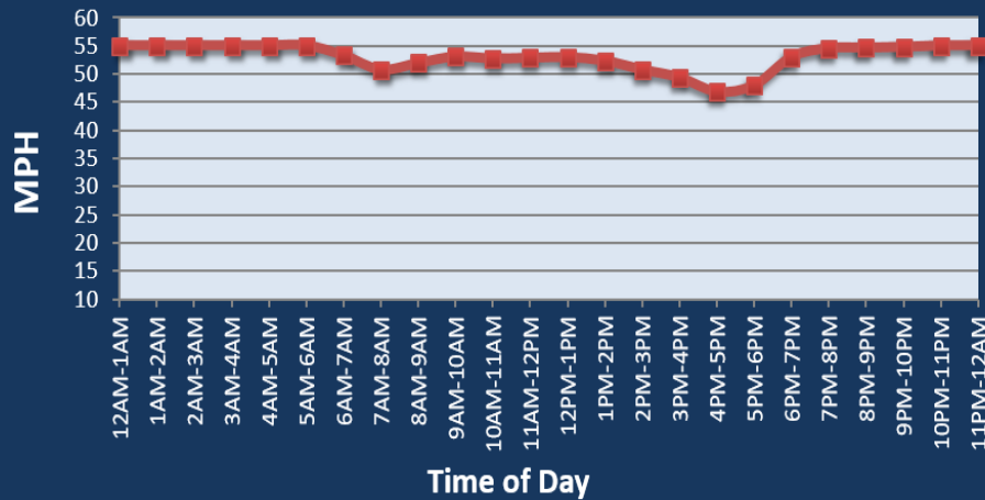
Average Speed by Time of Day SR 581 at I-83
