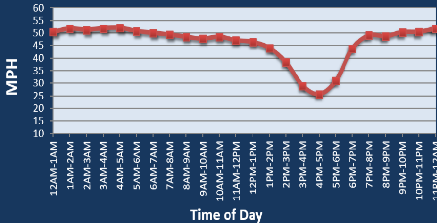
Average Speed by Time of Day I-376
