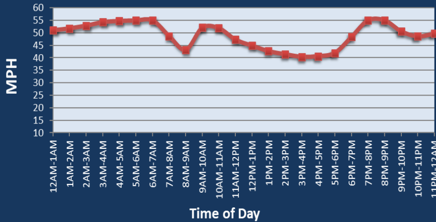
Average Speed by Time of Day I-75 at I-24
