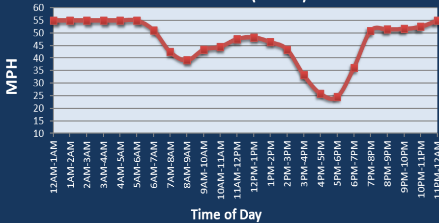
Average Speed by Time of Day I-24 at I-440 (North)
