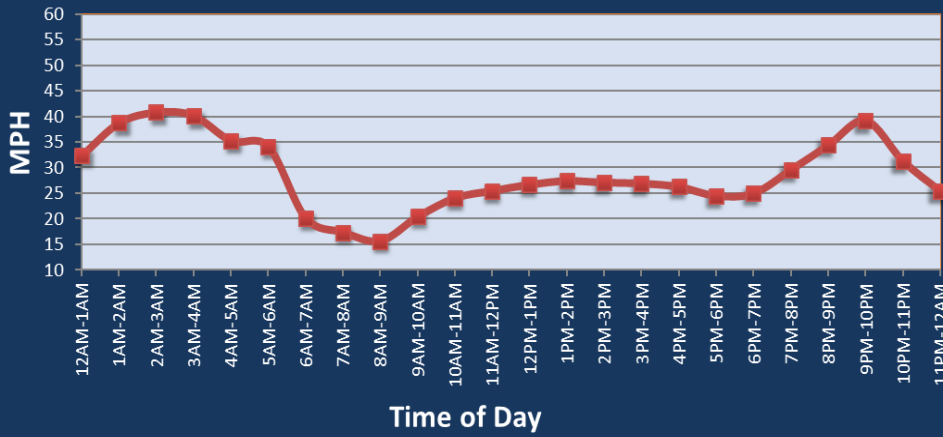
Average Speed by Time of Day I-95 at SR 4
