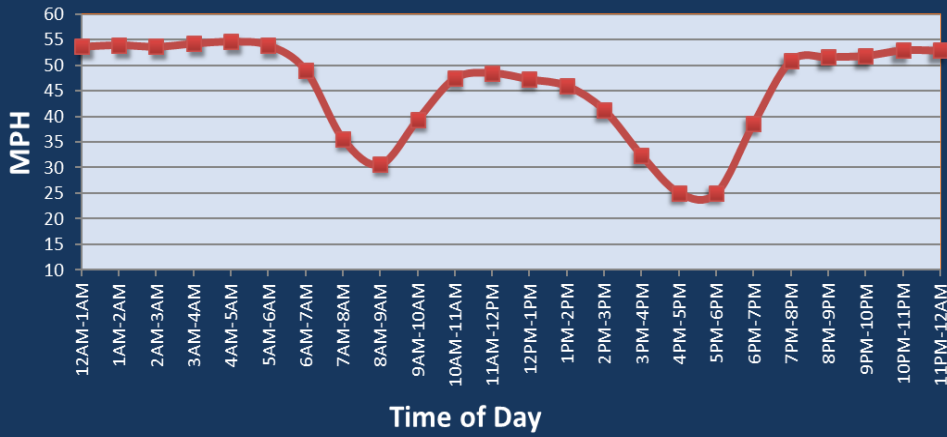
Average Speed by Time of Day I-26 at I-526
