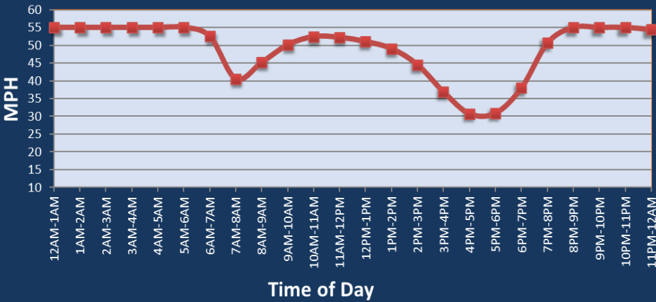
Average Speed by Time of Day I-287
