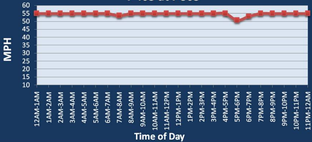
Average Speed by Time of Day I-465 at I-865
