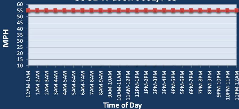
Average Speed by Time of Day US 31 W at SR 9001/I-65
