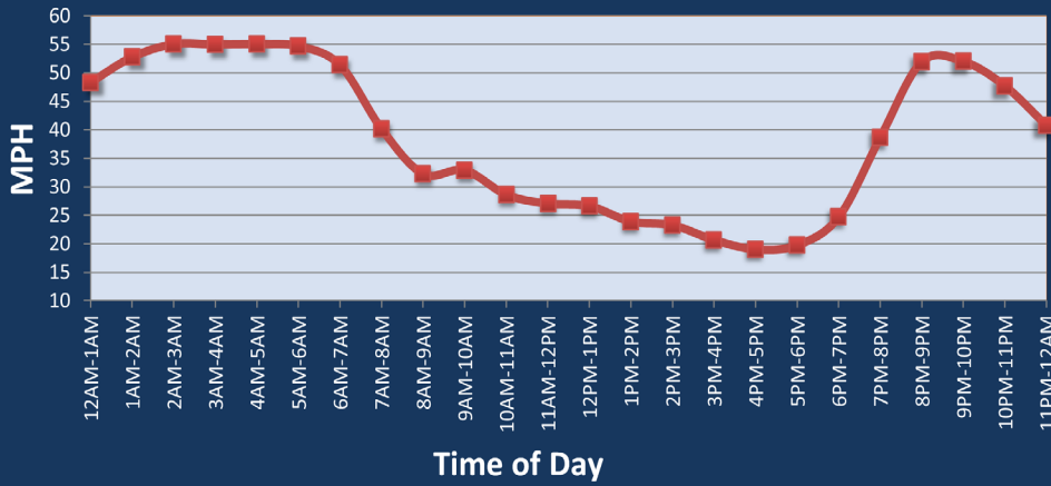
Average Speed by Time of Day I-495 (West Side)
