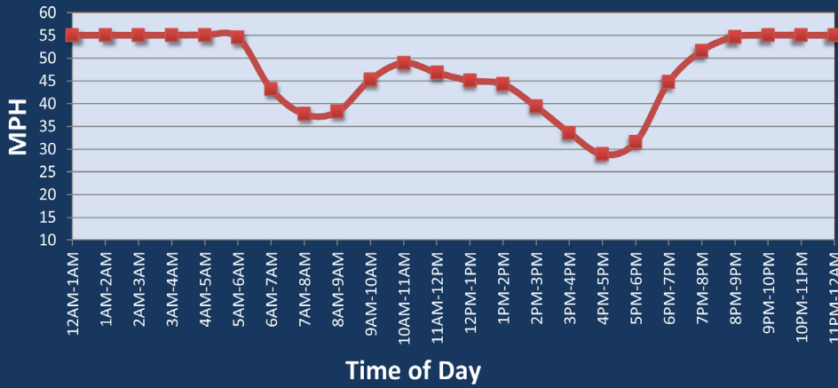
Average Speed by Time of Day I-70 at I-270
