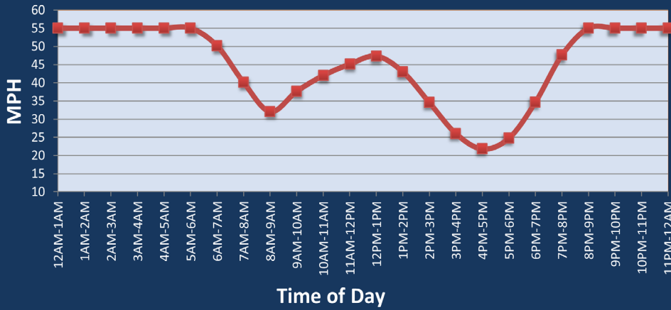
Average Speed by Time of Day I-495 at I-270 (West)
