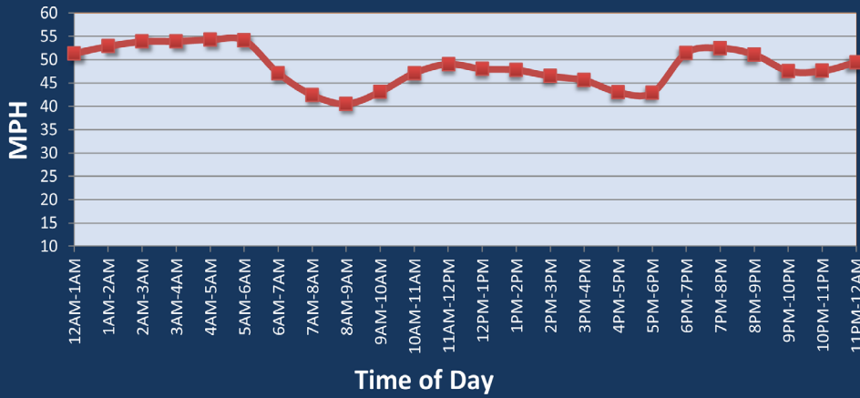
Average Speed by Time of Day I-80 at US 50
