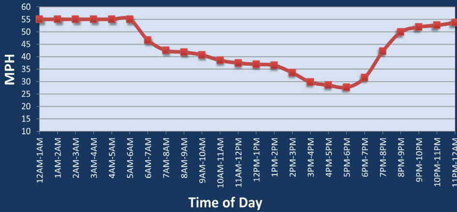
Average Speed by Time of Day I-20 at I-285 (West)
