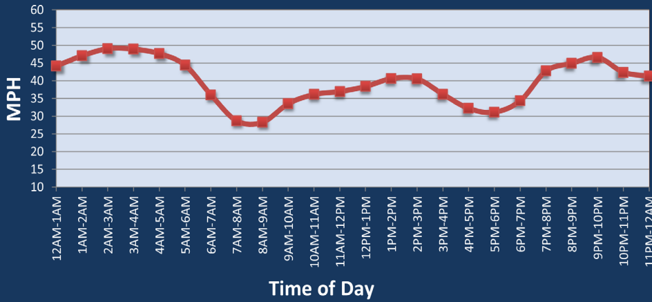
Average Speed by Time of Day I-278 at Belt Parkway
