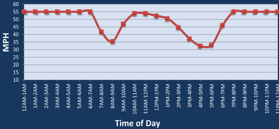
Average Speed by Time of Day I-80 at I-5
