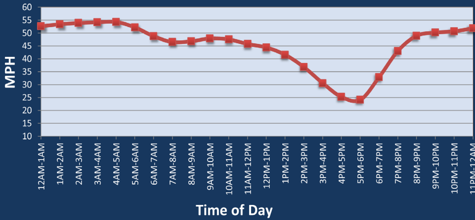
Average Speed by Time of Day I-71 at I-75
