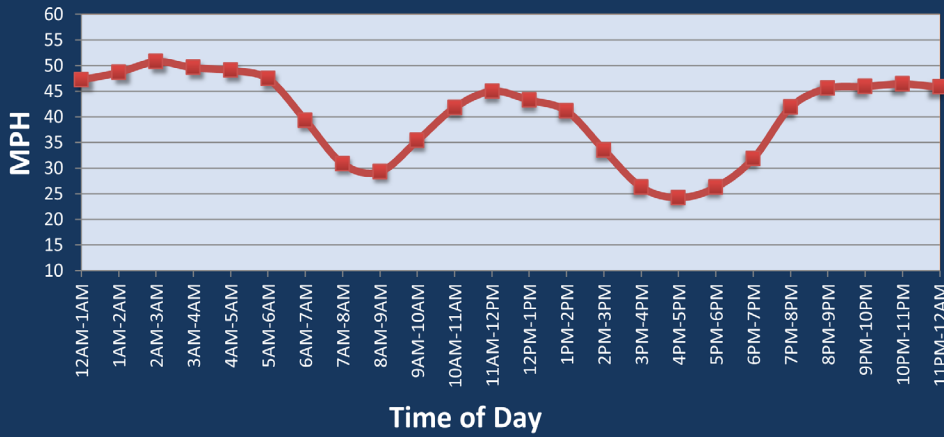
Average Speed by Time of Day I-110 at I-105
